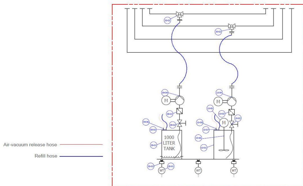
Figure 1: Ex. on an Easy Weigh Unit flow-diagram / flow-process.
